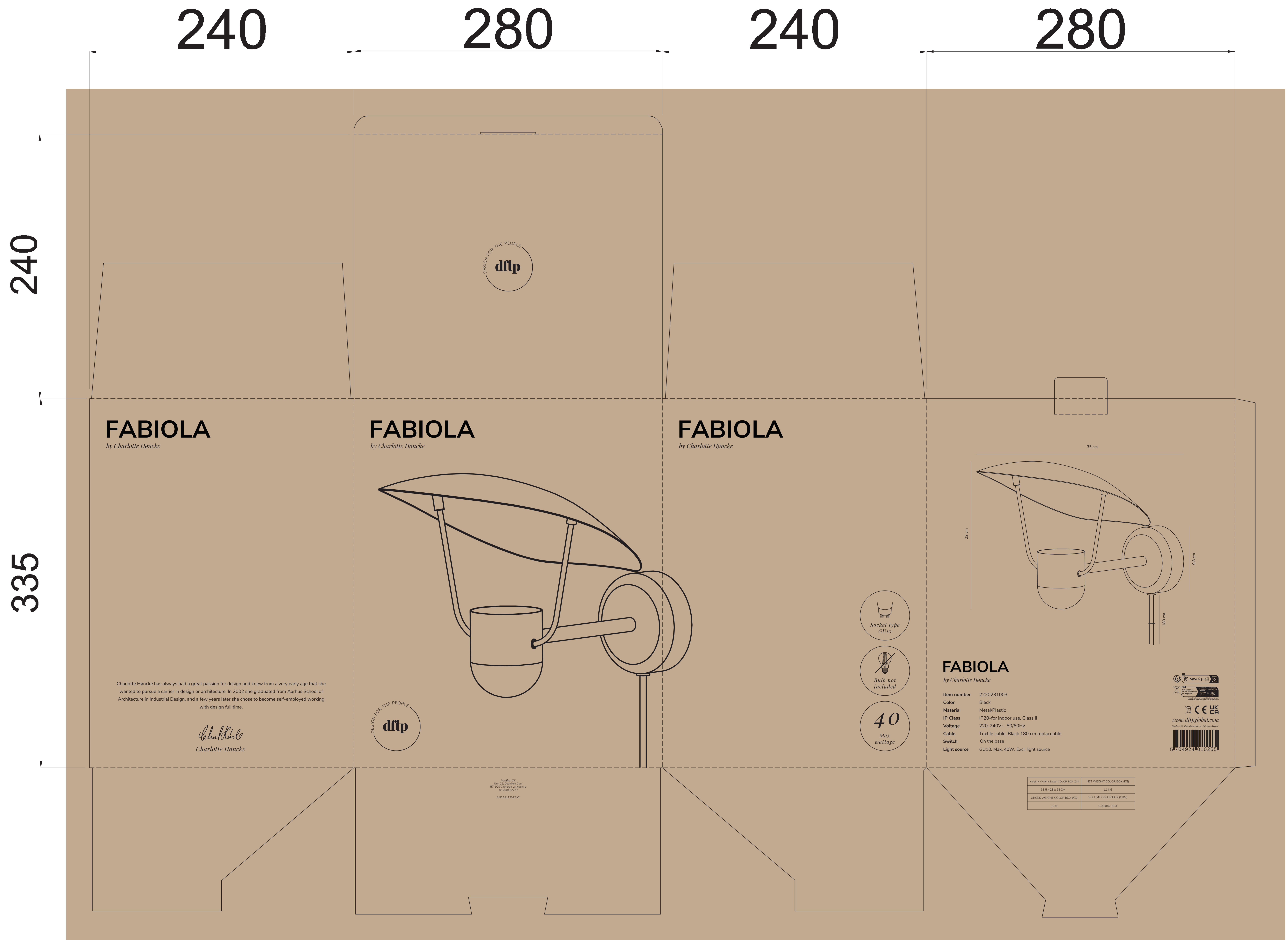
2220231003 Wall(B flute) interbox /1pcs: 280x240x335 mm
