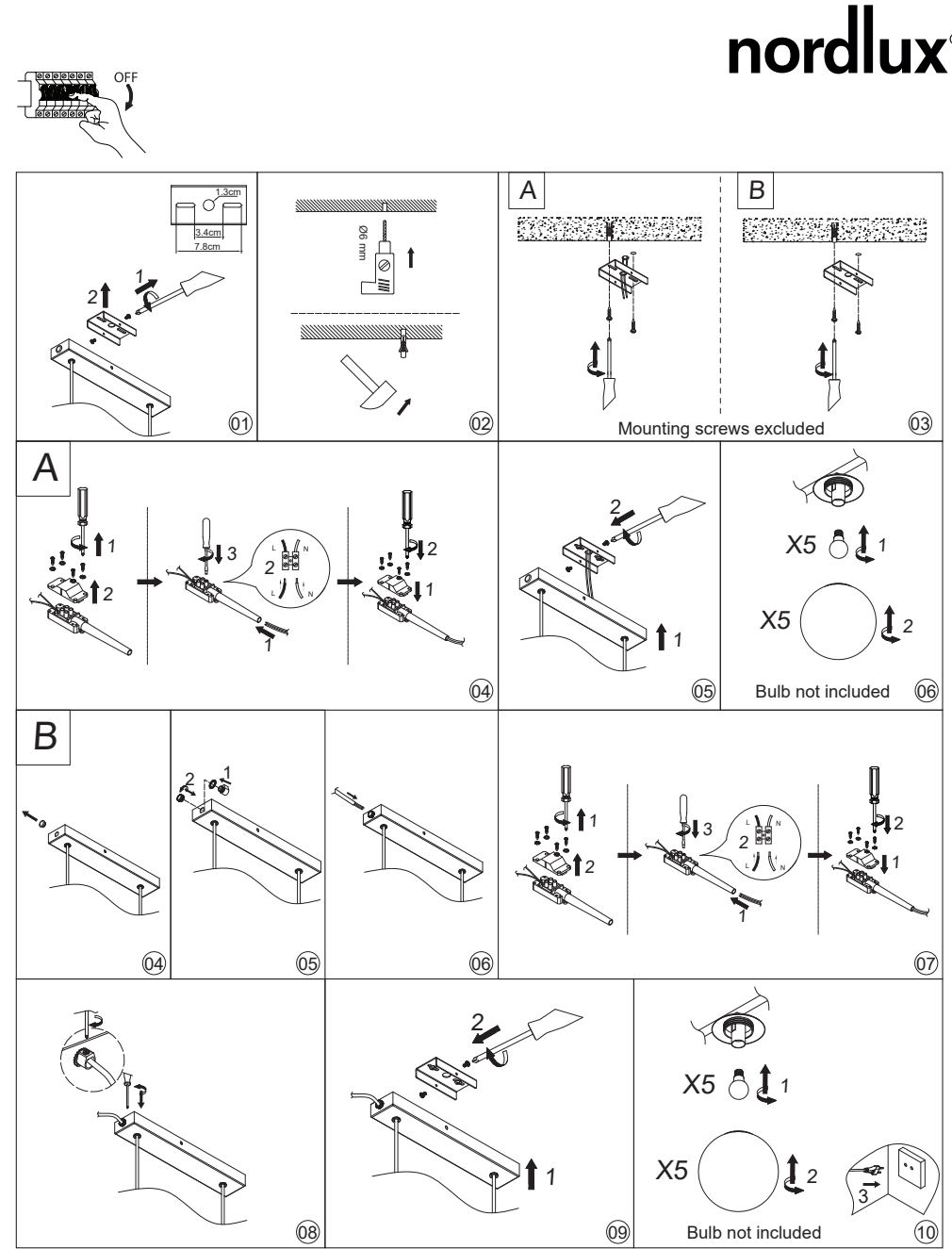
CE UKCA Monteringsanvisning | Montageanleitung | Mounting instruction | Installationsanvisningar | Instructions de montage | Montage-instructies | Item Nr.: 261262
