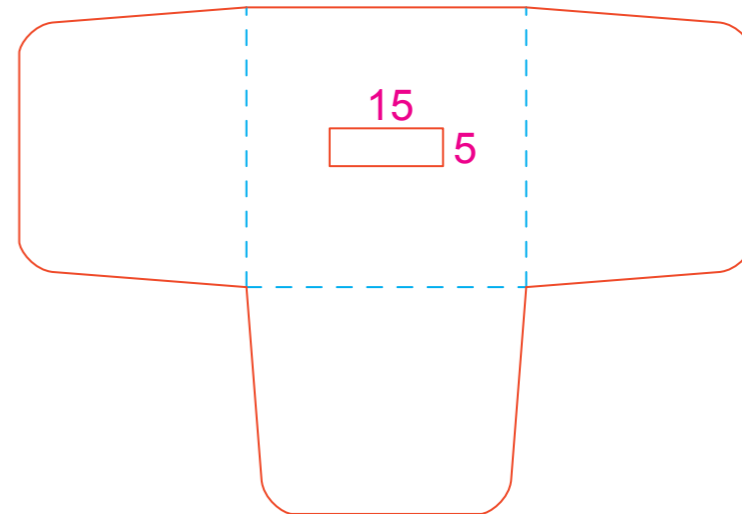
400g灰底白板纸37×37×30mm 展开尺寸97×67mm
